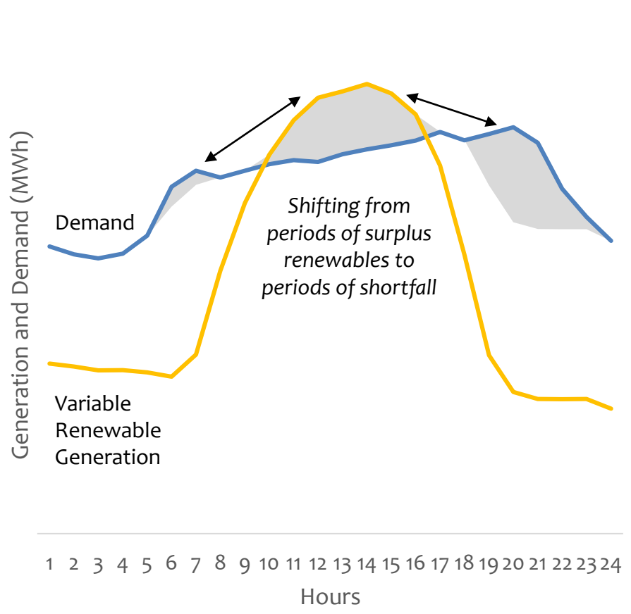
Intraday/Daily Balancing and Shifting
