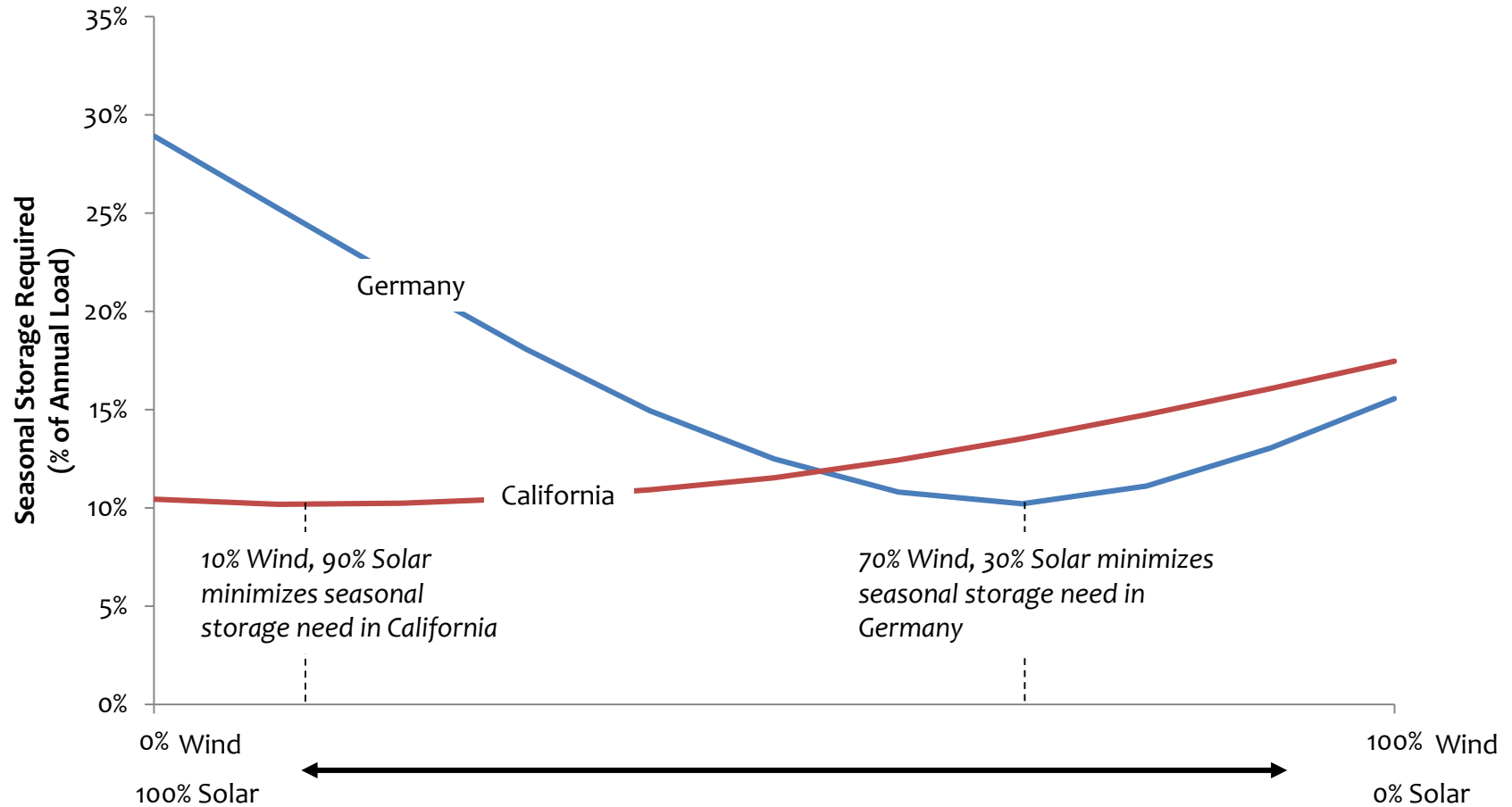
Cumulative interday/seasonal storage required for different shares of wind and solar % of annual MWh
